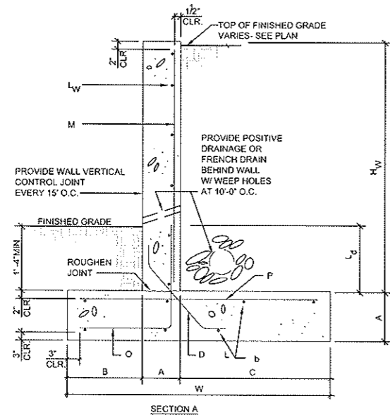
B TYPICAL RETAINING WALL SECTION A CONC/WALL001
