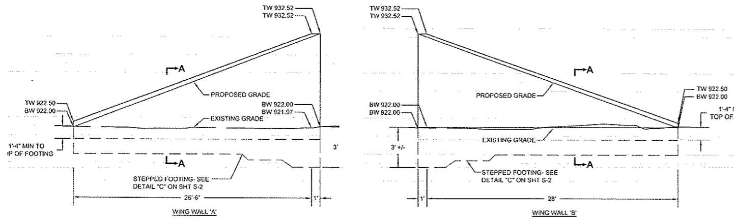
A WING WALL ELEVATIONS S-2
