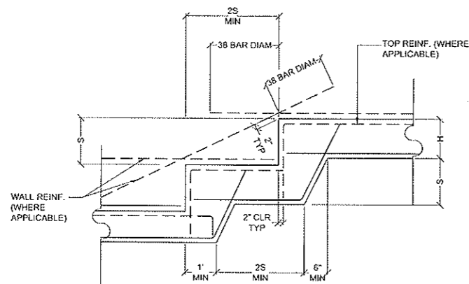
C TYPICAL STEPPED FOOTING DETAIL S-2
